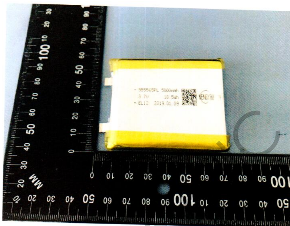
Figure 1 Overall view I of cell (外观图I)
